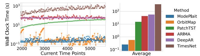
Figure 3: Scalability of MODEPLAIT: (left) Wall clock time vs. data stream length t_c and (right) average time consumption for (#4) exercise. The vertical axis is a logarithmic scale.
